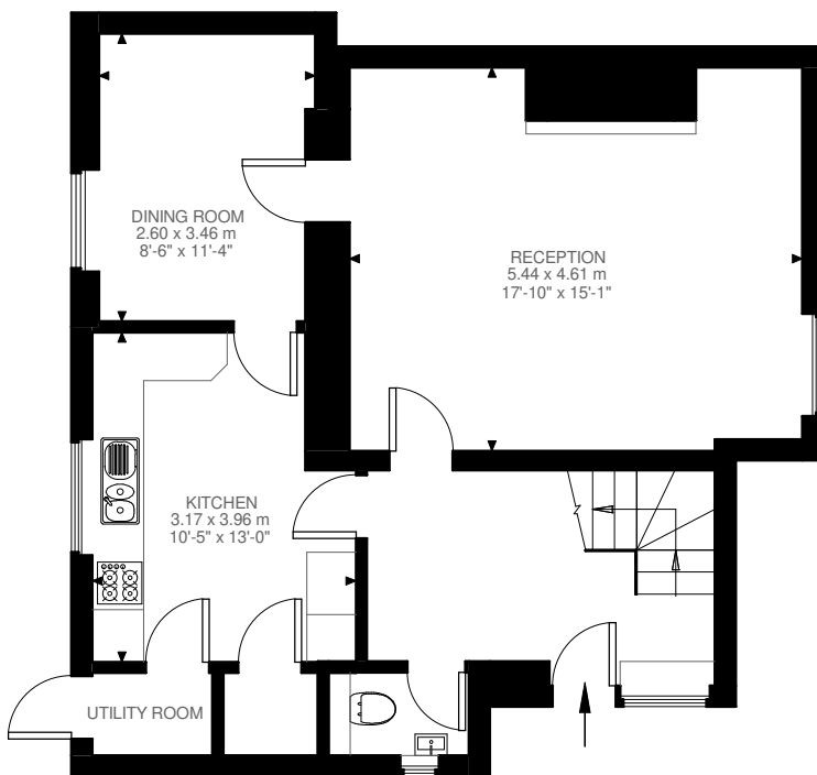
Ground Floor 706 ft 2
